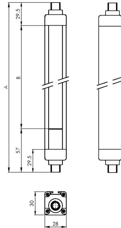
EOS4 Master - EOS4 Slave2 (Emisor y Receptor)
